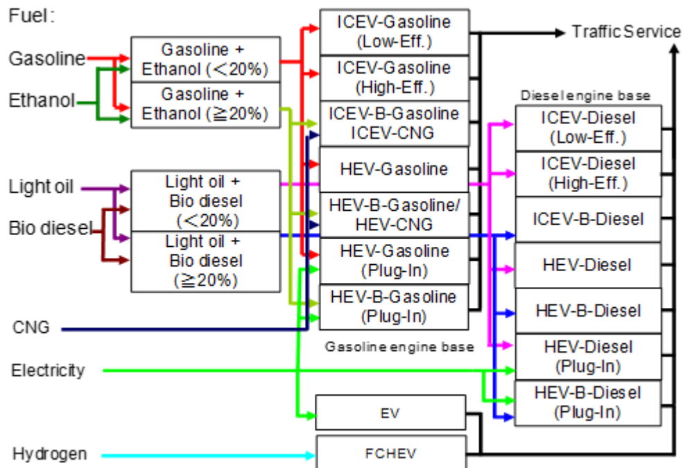
Figure 22 Taxonomy of passenger cars in DNE21+
