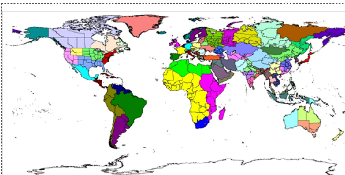
Figure 2 DNE21+ 77 regions
