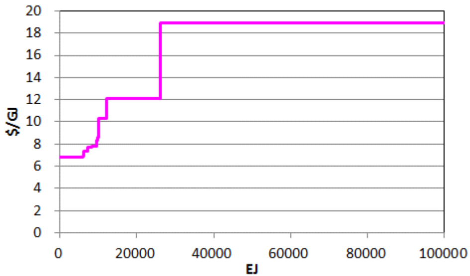
Figure 9 Cumulative Global Oil Supply Curve (incl. Non-conventional)
