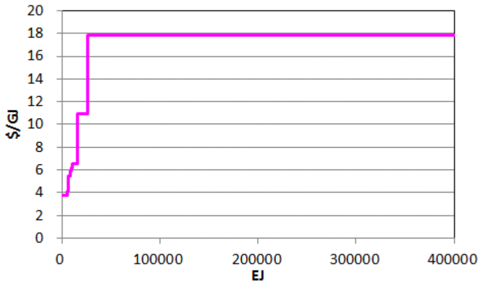
Figure 10 Distribution of Conventional Natural Gas Resources (Source) USGS
