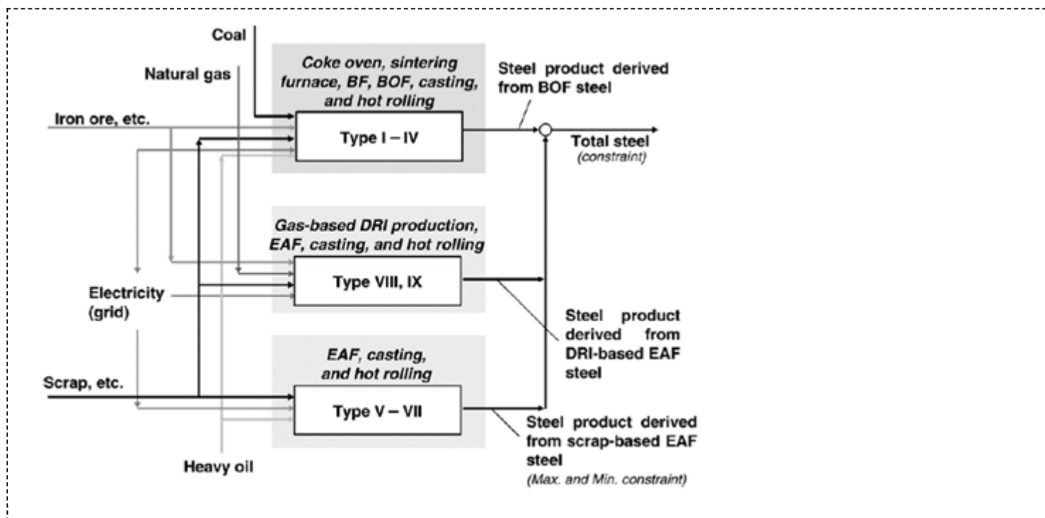
Figure 25 Modeling of energy use of the steel sector in DNE21+.
